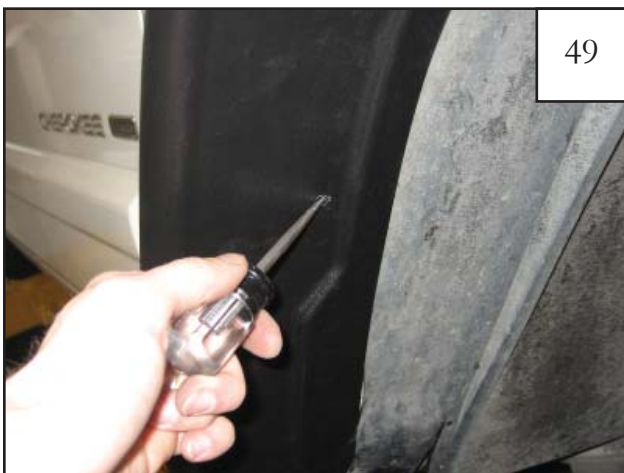
Use a scratch awl (or another pointed tool) to line up the speed clips with the outer flare holes (6 locations). If needed, use a flashlight to better locate the speed clips.
