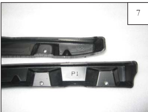
Locate the flat style flare passenger side front inner pieces marked P1 & P2. The driver side front inner pieces are marked D1 & D2.
