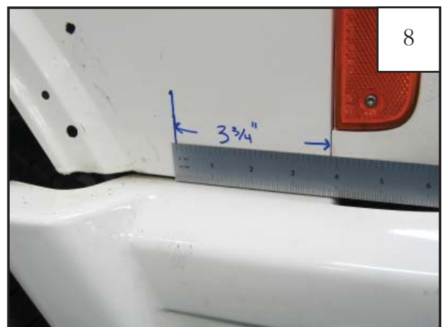
Use a grease pencil or removable marker to mark a vertical line 3-3/4" from the front edge of the sheet metal on the fender.
