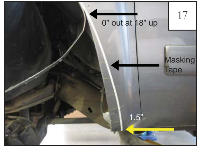
17 At the bottom of cut fender, measure 1.5" toward door seam and make a mark. Use masking tape to created a reference line from mark at bottom up to the 18" point.
