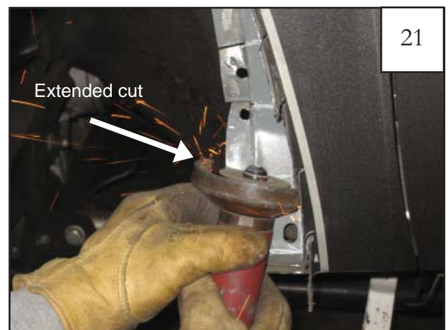
21 Continue cutting flange at existing cut lines, stopping at the line parallel to the inner wall.
