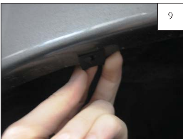
Install #10 U-Clip (CL1-0022) over existing factory holes.
